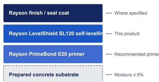
Figure 1 — Typical system build-up (top to bottom). Layer thicknesses are system-dependent; confirm the specification for your project.
