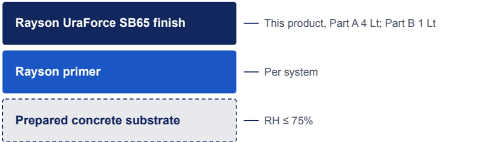
Figure 1 — Typical system build-up (top to bottom). Layer thicknesses are system-dependent; confirm the specification for your project.
